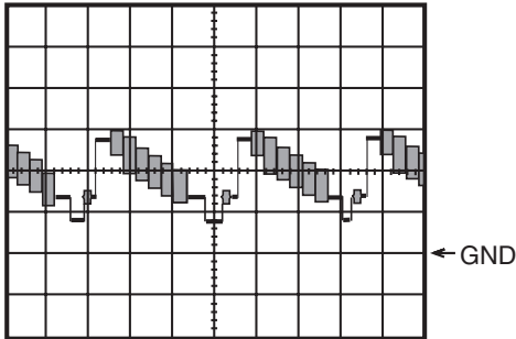
WF1 1DIV: 0.5V 20 \mu sec IC 111 Pin 26
